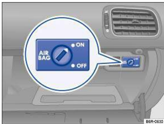
Fig. 62 In the stowage compartment on the front passenger side: key switch for disabling and enabling the front airbag on the front passenger side
